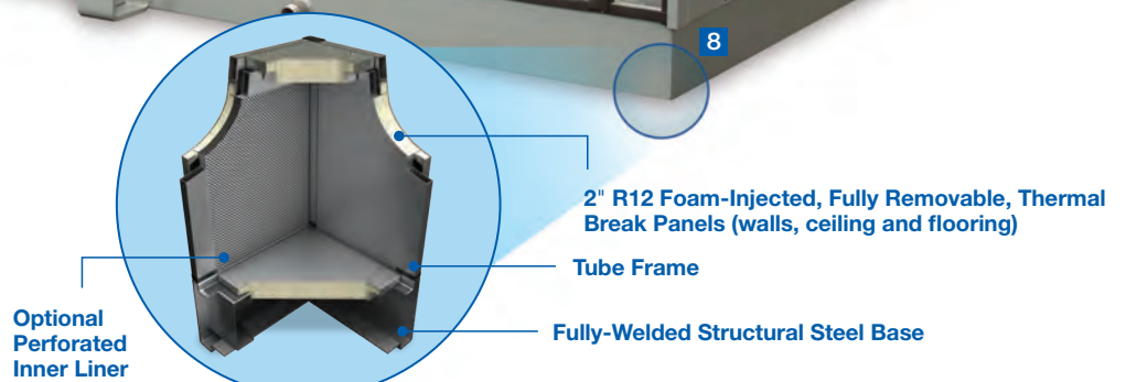
Standard Casing
